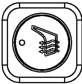
SWITCH CHECK CORP P/N SW-SPST-33-12V FRONT VIEW
